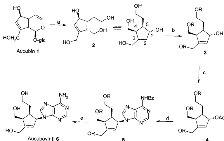
Scheme 1. R = isobutyryl; Bz = benzoyl; (a) (i) \text{Hg}(\text{OAc})_2 , \text{NaBH}_4 , or (ii) \beta -glucosidase, \text{NaBH}_4 , 90%; (b) isobutyric anhydride, pyridine, 0 °C \rightarrow 25 °C, 1.5 h, 90%; (c) \text{Ac}_2\text{O} , pyridine, 1 h, 99%; (d) (i) N 6 -benzoyl-adenine, \text{CH}_3\text{CN} , \text{TMSCl} , \text{HMDS} , (ii) \text{CF}_3(\text{CF}_2)_3\text{Si}(\text{CH}_3)_3 , \text{CH}_2\text{Cl}_2 , reflux, 8 h, 20%; (e) \text{DIBAL} , \text{CH}_2\text{Cl}_2 , -78 °C, 95%
