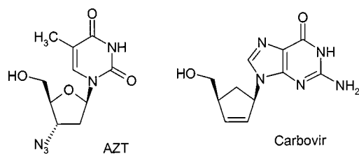
Figure 1. Nucleoside analogs
