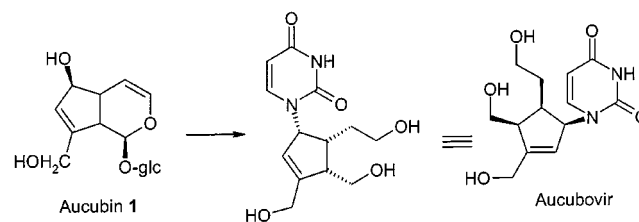
Figure 2. Synthesis of Aucubovir
